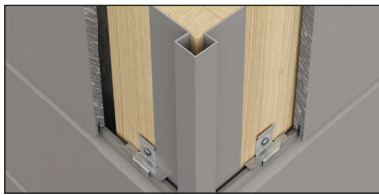
Picture 1 Swisspearl External Corner Profile Small
