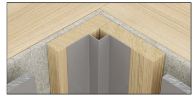
Picture 3 Swisspearl Internal Corner Profile
