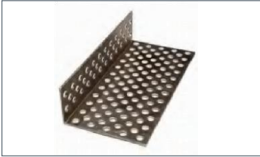
5. Swisspearl Internal Corner Profile 36x23x23mm coloured aluminium profile for 90° angle
